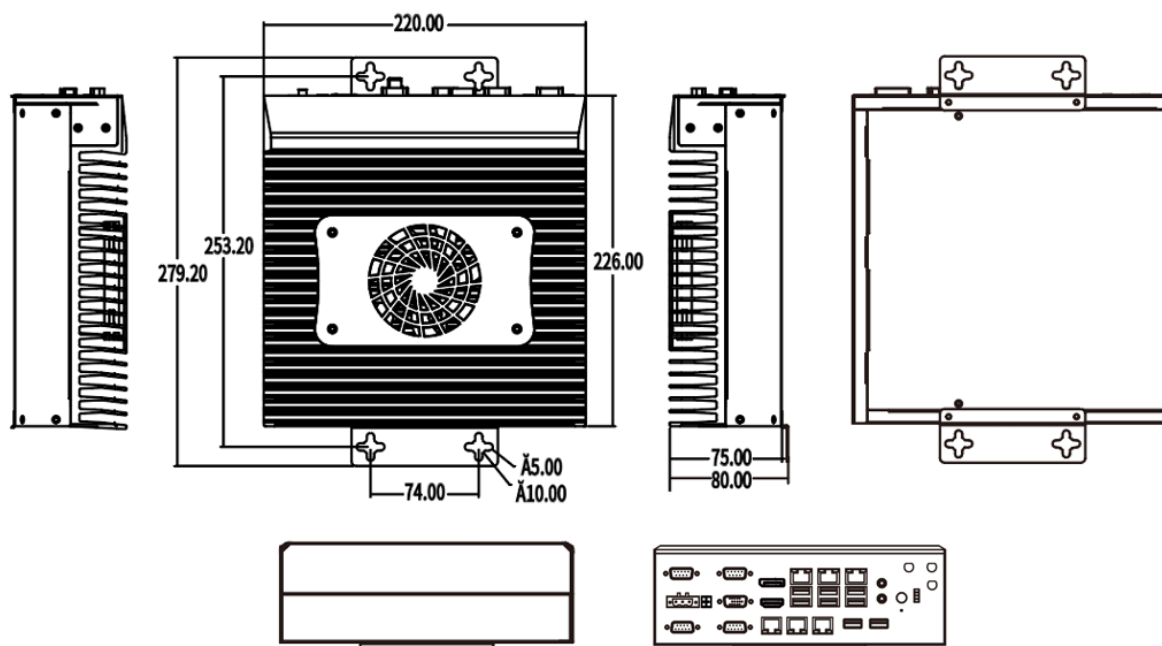
Figure 1-1 Dimension of the E512C-H610
